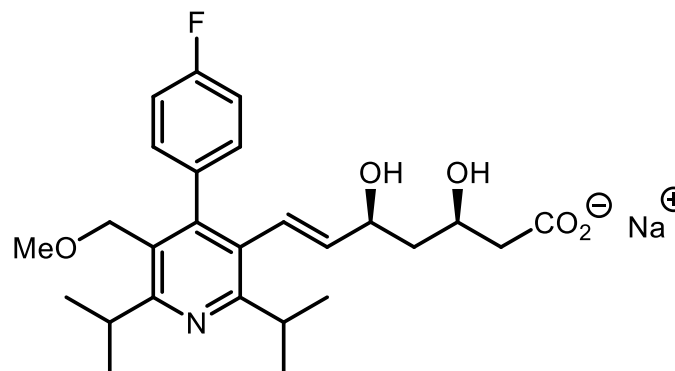
Cervivastatin (Lipobay®)
